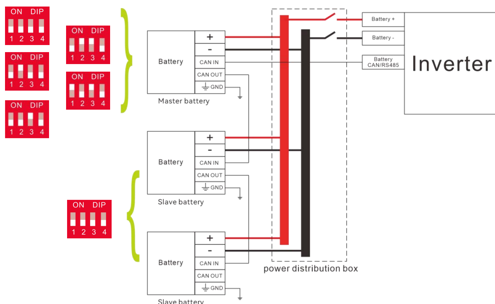
Figure 3-6 Wiring schematic diagram
