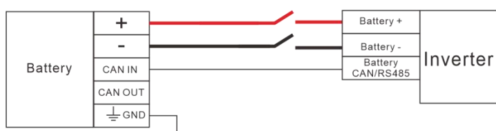
Figure 3-5 Wiring diagram
