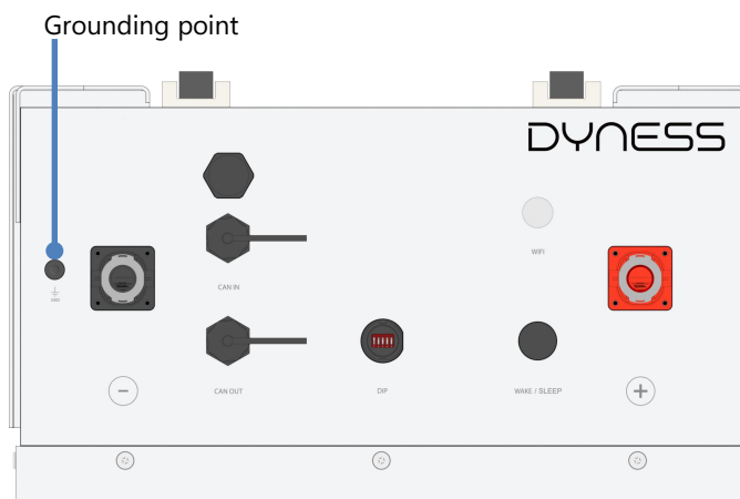
Figure 3-4 Location of grounding point
