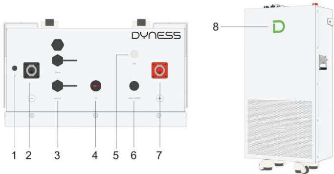
Figure 2-1 PowerBrick Pro the Sketch of Front Interface
