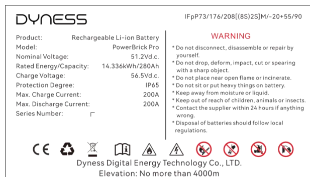
Figure 1-1 Battery Module Label
