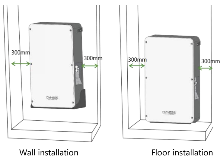
Figure 3-3 Mounting Space Requirements
