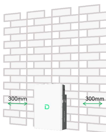
Floor installation
