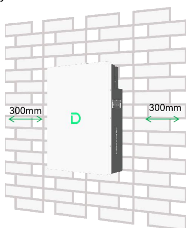
Wall installation
